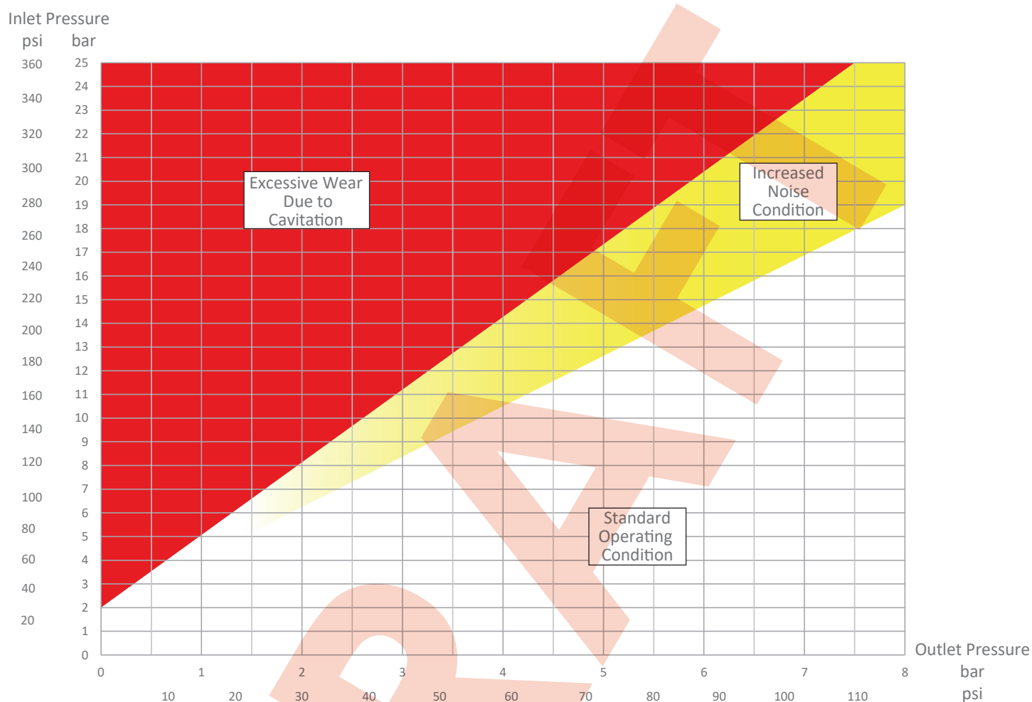
Cavitation Chart
