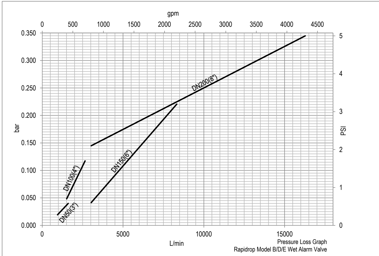
Pressure Loss Graph
